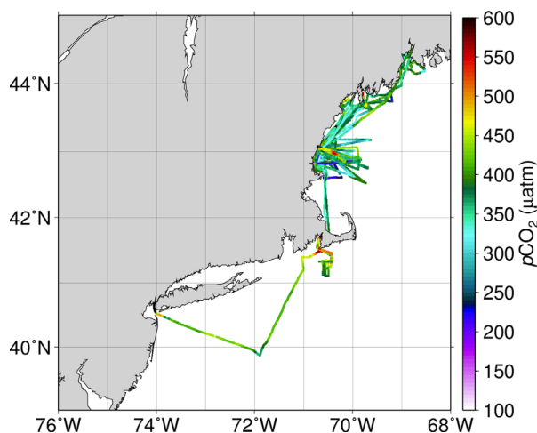
Figure A2. Map showing the underway p\text{CO}_2 tracks in the GoM and a single cruise track from Woods Hole to New York City.
