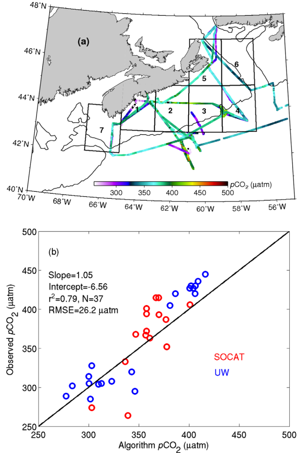
Figure 7. (a) Map showing the seven 2° × 2° boxes covering the entire Scotian Shelf (SS) region adapted from Shadwick et al. [2010]. The contour line is the 200 m isobath. The algorithm and in situ (SOCAT (not shown) and UW observations from Dalhousie University cruises) mean surface ocean p\text{CO}_2 were obtained for each of the seven boxes for evaluation purposes. (b) The scatterplot of algorithm versus observed p\text{CO}_2 for all seven boxes is shown with corresponding statistics in the legend.
