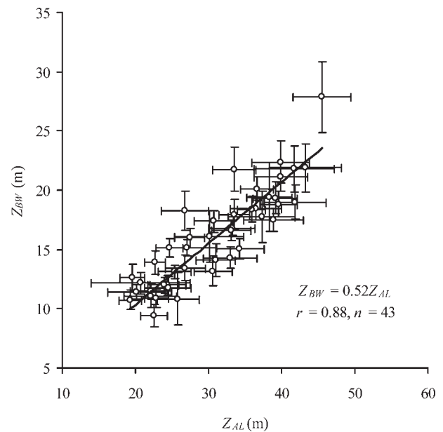
Fig. 2. Comparison between the depth of disappearance of the BW disk ( Z_{BW} ) and of the artificial light ( Z_{AL} ) that was used in the period 1949–1954. Each point represents the average depths ( \pm SE) of a geographical cell. The size of each of the 43 geographical cells was 2^\circ \times 2^\circ , and the cells were located from 24^\circ\text{N} to 44^\circ\text{N} . Each cell contained on average 18 observations for each of the two methods.
