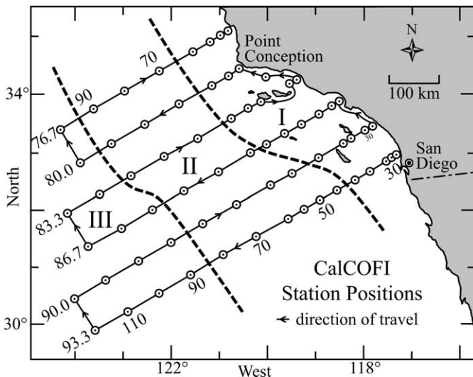
Fig. 1. CalCOFI sampling stations considered here. All observations were grouped according to their geographical position into three subareas: inshore (I), transition (II), and offshore (III). The dashed lines show the approximate border between these subareas (see text for details). Numerals to the left of each sampling line indicate the line number and numerals above or below the station locations indicate the station number.
