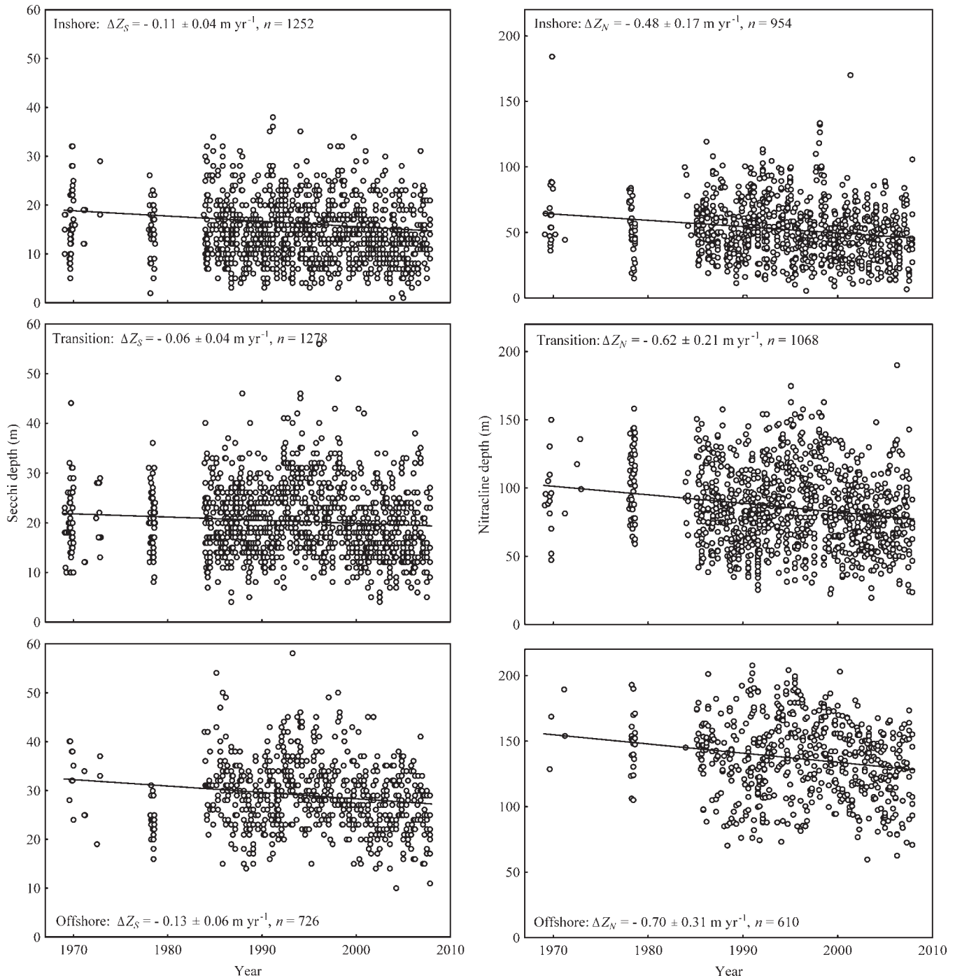
Fig. 3. Observations of Z_S (Secchi depth, left panel) and Z_N (nitracline depth, right panel) in the inshore, transition, and offshore areas of the southern sector of the CCS (see Fig. 1). The average annual changes ( \pm 95\% confidence intervals) in the Secchi ( \Delta Z_S ) and nitracline ( \Delta Z_N ) depths were estimated by linear regression where n is the number of observations. For both variables in all three areas a significant ( p < 0.01 ) overall shoaling (negative slopes) was measured.
