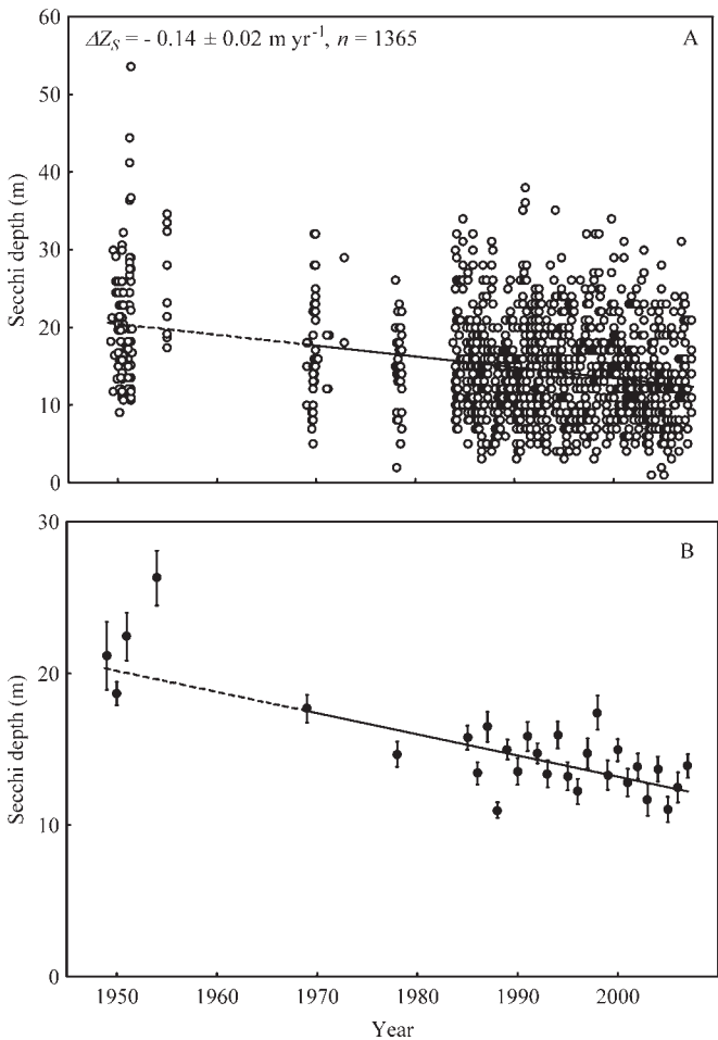
Fig. 5. (A) Secchi depth observations of the inshore area over the time period 1949–2007. Note that the observations from 1949–1954 are calibrated BW-disc observations (see Methods for details). The average ( \pm SE) annual shoaling rate ( \Delta Z_S ) was estimated with linear regression analysis where n is the number of observations. (B) Temporal changes in annual mean Secchi depth.
