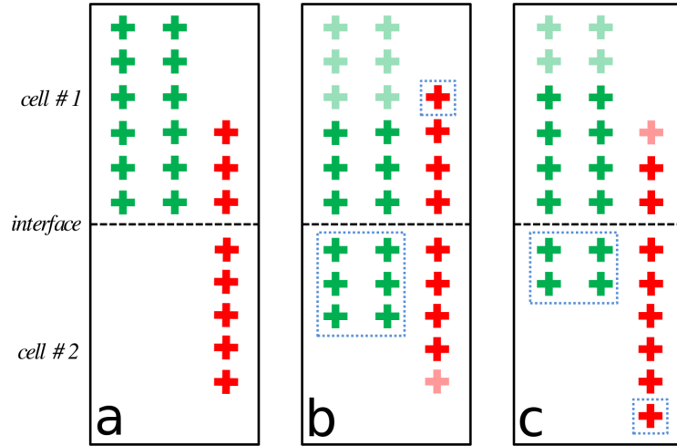
Figure 2.1: Schematic representation of the difference between the treatment of diffusion within the traditional TBNT approach (Ménésguen and Hoch, 1997) and the adapted approach used in this study. The panels show the distribution of two fraction variables of the same species (red/green crosses) at (a) initial state and after instantaneous mixing according to (b) the traditional and (c) the adapted approach. Light-coloured crosses represent the original location of particles which have been diffusively transferred to their target location (blue dotted boxes).
